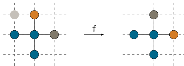
Figure 5: Local isometry that can not coincide with a global isometry on its entire domain of definition
