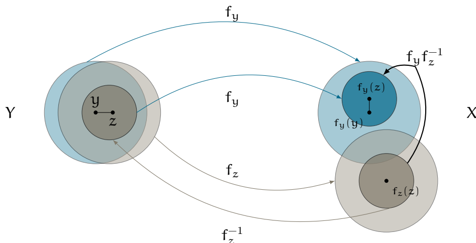
Figure 8: Composition of isometries with neighbouring centers
