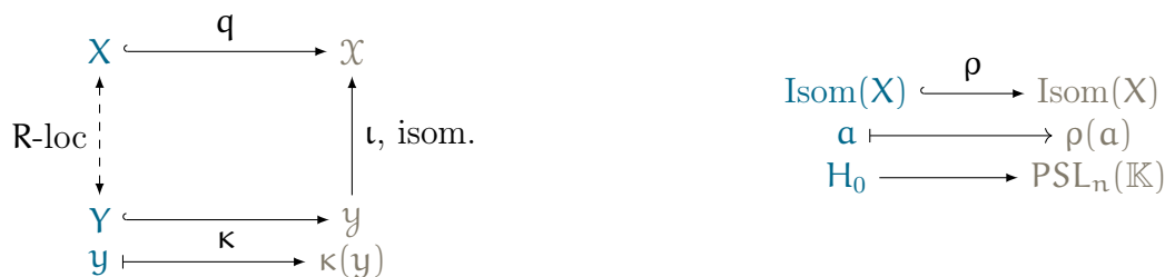
(a) Maps between graphs
