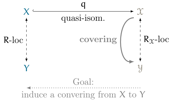
Figure 2: Sketch of the proof
