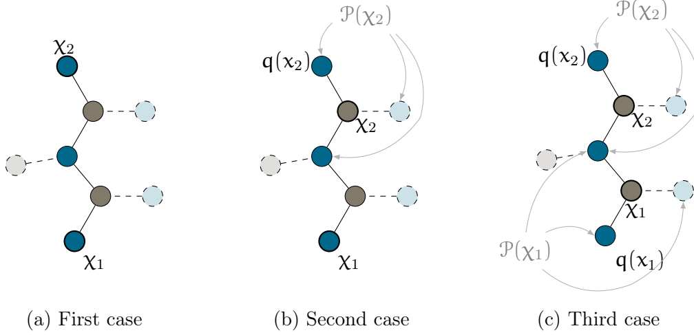
Figure 11: The three cases ( \text{im}(q) is represented by the blue vertices)
