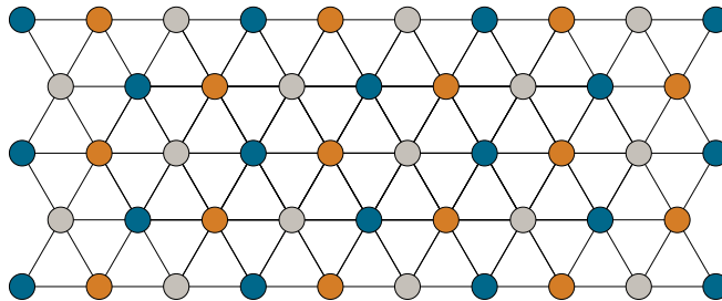
Figure 4: Apartment in the building of \mathrm{PSL}_3(\mathbb{Q}_2) . The colors correspond to \mathrm{SL}_3(\mathbb{Q}_2) -orbits.
