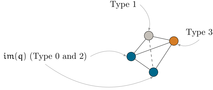
Figure 6: Partition of a simplex
