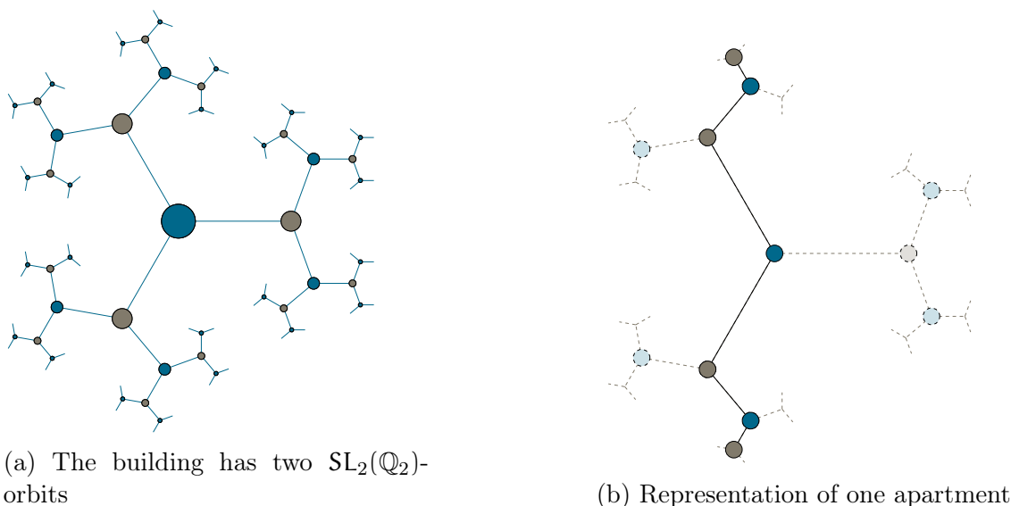
Figure 3: The building of \mathrm{PSL}_2(\mathbb{Q}_2)
