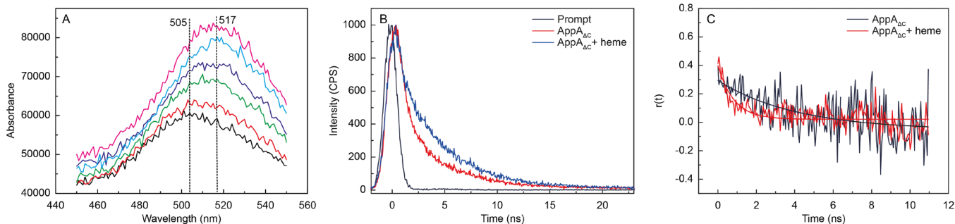
Fig. 5 (A) Shift of the fluorescence emission maxima of the dark-adapted AppA _{\Delta C} at increasing heme concentrations. (B) Fluorescence decay of the dark-adapted AppA _{\Delta C} in the absence (red) and presence of heme (blue) after excitation at 455 nm, ( \lambda_{em} = 520 nm). The instrument response function ( \sim 1 ns) is shown in black. (C) Decay of the fluorescence anisotropy of the dark-adapted AppA _{\Delta C} in the absence of heme (black) and in the presence of heme (red). Fits are shown as solid traces.
