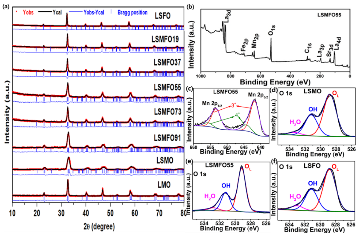
Fig. 1 a) XRD profile with Rietveld refinement of unsubstituted and substituted \text{LaMnO}_3 perovskites; b) XPS survey spectrum of LSMFO55; c) XPS Mn 2p spectrum of LSMFO55; d-f) O 1s spectrum corresponding to LSMO, LSMFO55 and LSFO, respectively.
