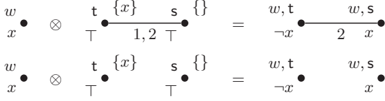
Figure 1: Epistemic model M (left) for which x \in V(1), x \notin V(2) , action models \langle \{x\} \uplus T! \rangle (top) and \langle \{x\} \cup T! \rangle (bottom), and the resulting model products (right).
