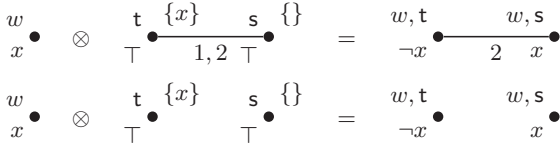
Figure 1: Epistemic model M (left) for which x \in V(1), x \notin V(2) , action models (\dagger x \cup T!) (top) and (\dagger x \cup T!) (bottom), and the resulting model products (right).
