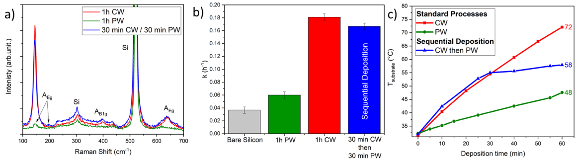
Figure 8 : Raman spectra (a), MB degradation rate under UV (365 nm, 2 mW/cm 2 ) (b) and sample temperature evolution as a function of deposition time (c)
