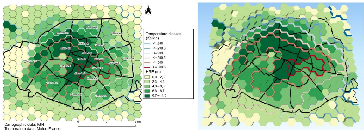
Figure 20: 2D co-visualization of simulated air temperature data with one morphological indicator
