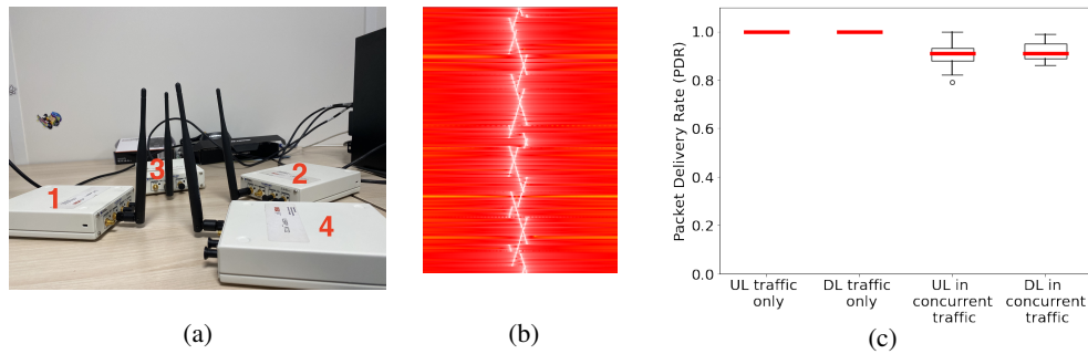
FIGURE 1: (a) Testbed setup using four USRPs. (b) Waterfall diagram for two concurrent uplink and downlink frames, with time flowing downwards. (c) PDR for uplink and downlink traffic. The boxes show the median (in red), the first and third quartile (the box), and the 95% confidence interval (the whiskers).
