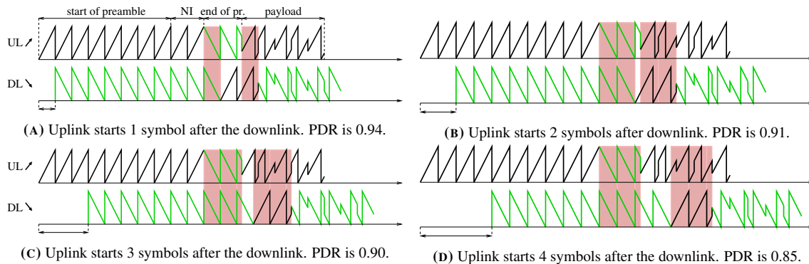
FIGURE 2: Concurrent uplink and downlink transmissions as a function of the time offset between the two frames. The red boxes represent collisions between upchirps (in black) and respectively downchirps (in green) from different frames. The PDR is computed as the mean between uplink and downlink PDRs in the specified setup.
