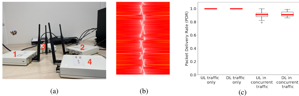
FIGURE 1: (a) Testbed setup using four USRPs. (b) Waterfall diagram for two concurrent uplink and downlink frames, with time flowing downwards. (c) PDR for uplink and downlink traffic. The boxes show the median (in red), the first and third quartile (the box), and the 95% confidence interval (the whiskers).
