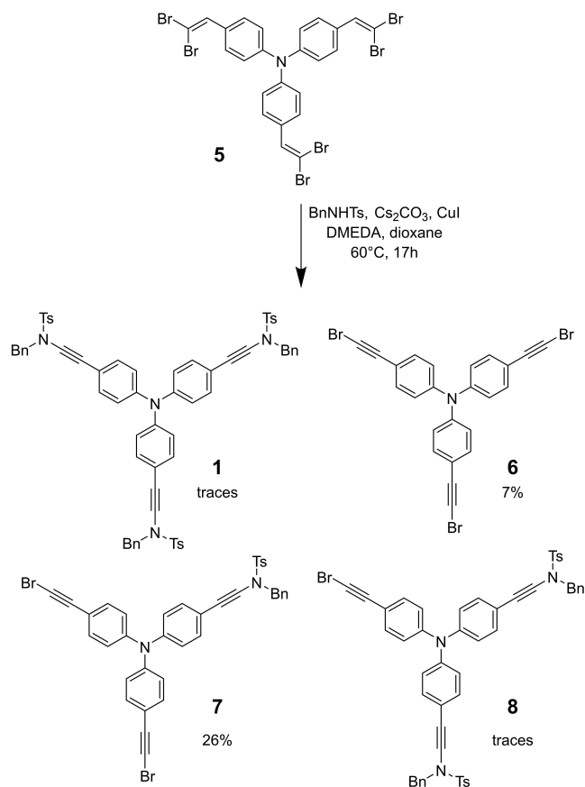
Scheme 1. Reaction of compound 5 with benzyltosylamide under Evano's conditions.
