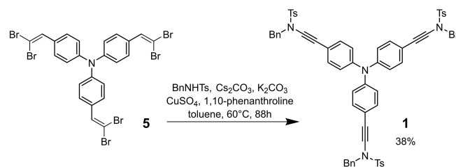
Scheme 2. Reaction of compound 5 with benzyltosylamide under Hsung's conditions for the successful synthesis of tris-ynamide 1 from compound 5 .
