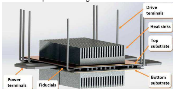
Figure 2: agile Power Switch 3D-Integration power module
