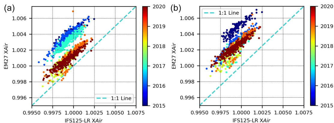
Figure 22. Correlations for the retrieved X_{\text{AIR}} by using the instrument SN37 and IFS125-LR. Panel (a) shows the results of the analysis of atmospheric spectra under the assumption of a constant ILS, and (b) shows the results under the assumption of a variable ILS (ILS parameters adjusted on a yearly basis).
