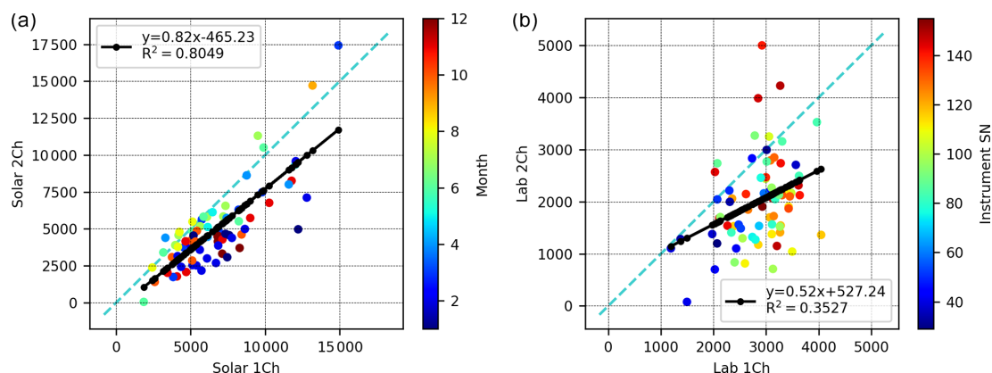
Figure 26. Correlations of the SNR obtained in channels 1 and 2, for the solar and OP measurements in (a) and (b), respectively. In (a) the colour code represents the month of the year when the solar measurements were carried out, for demonstrating the absence of an obvious seasonal signal in the SNR characteristics. In (b), the colour code represents the instrument's serial number because these measurements are carried out under controlled laboratory conditions by using a lamp as a light source. There might be a slight tendency towards higher SNR in recently built spectrometers.
