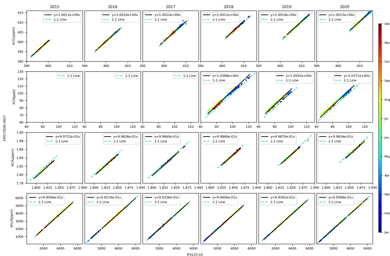
Figure 23. Correlations between the species: \text{XCO}_2 , \text{XCO} , \text{XCH}_4 and \text{XH}_2\text{O} retrieved with the COCCON reference instrument and the TCCON instrument in low-resolution measurement mode in each row (top-down), respectively, treated separately by year from 2015 to 2020 in each column for each species.
