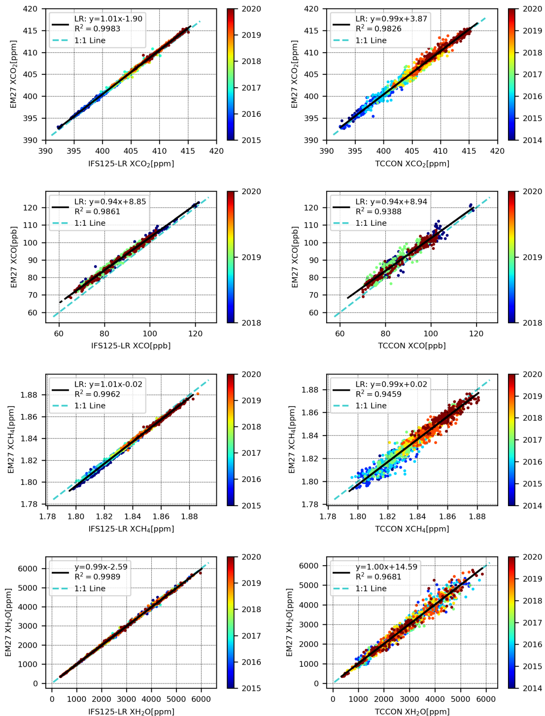
Figure 21. Correlations between \text{XCO}_2 , \text{XCO} , \text{XCH}_4 and \text{XH}_2\text{O} between the ones retrieved by using the COCCON reference and the IFS125-LR low-resolution data (left panels) and between COCCON reference and TCCON station (right panels).
