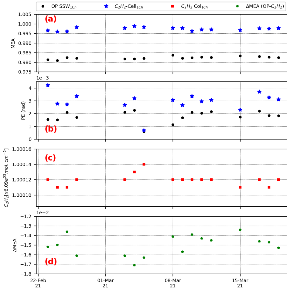
Figure 15. Time series of the MEAs, PEs, C_2H_2 retrieved column and difference between the MEAs retrieved with OP and cell method for the COCCON reference instrument SN37 (a, b, c and d, respectively).
