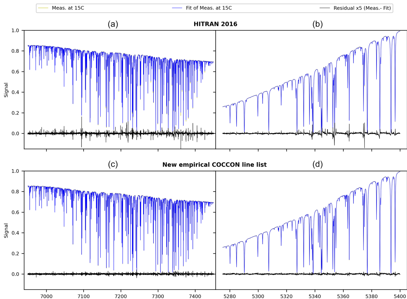
Figure A1. \text{H}_2\text{O} spectroscopic lines used for this ILS calibration study. The fits (multi-spectrum fit performed) using HITRAN 2016 and the new empirical COCCON line list are presented in (a, b) and (c, d), respectively. The measured spectra were taken with the IFS125HR at KIT Karlsruhe, at 15 °C. The spectral residuals shown are multiplied by 5 in order to be visible.
