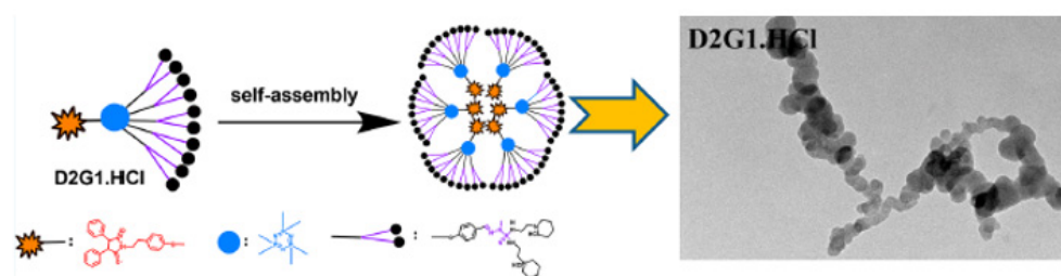
Figure 8. Self-assembly of \text{D2G1.HCl} amphiphilic dendrons to form nanostructured aggregates (micelles). Reproduced with permission from reference [39], American Chemical Society.
