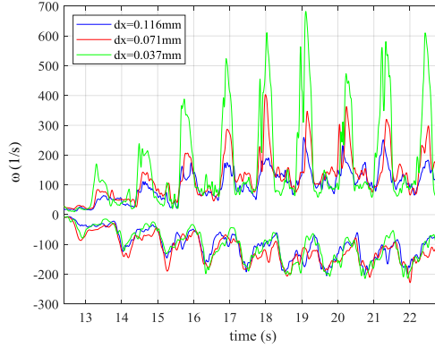
FIGURE 10. Comparison of the measured vorticity maxima using different field of views and pixel sizes for T = 1.1 s and H/\lambda = 1.6 %.
