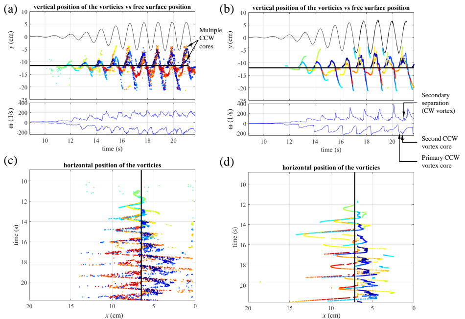
FIGURE 7. Vertical and horizontal positions of the vorticity maxima in the gap measured for case II (panels (a) and (c)) and computed using mesh case A (panels (b) and (d)) for T = 1.1 s and H/\lambda = 1.6\% . The colour range corresponding to the intensity of the vorticity is consistent with figure 6. The free surface elevation in the gap and the edges of the hull are shown by the respective thin and thick solid lines. The vorticity intensity is also shown in panels (a) and (c) for reference.
