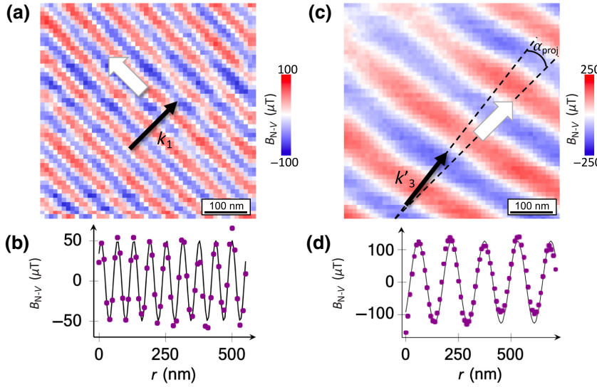
FIG. 5. (a) Quantitative stray-field map of the type-I cycloid in \text{BiFeO}_3/\text{DyScO}_3 . (b) Extracted and fitted line profile of the type-I cycloid. (c) Quantitative stray-field map of the type-II cycloid in \text{BiFeO}_3/\text{SmScO}_3 . (d) Extracted and fitted line profile of the type-II cycloid.
