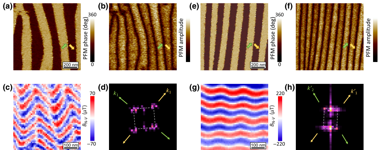
FIG. 2. In-plane PFM (a) phase and (b) amplitude images of the \text{BiFeO}_3 thin film grown on \text{DyScO}_3(110) . (c) Quantitative scanning N-V magnetometry image on the same sample and (d) corresponding FT. In-plane PFM (e) phase and (f) amplitude images of the \text{BiFeO}_3 thin film grown on \text{SmScO}_3(110) . (g) Quantitative scanning N-V magnetometry image on the same sample and (h) corresponding FT. Green and yellow arrows indicate the two in-plane polarization directions (wide arrows) and the corresponding k propagation vectors of the spin cycloids (thin arrows).
