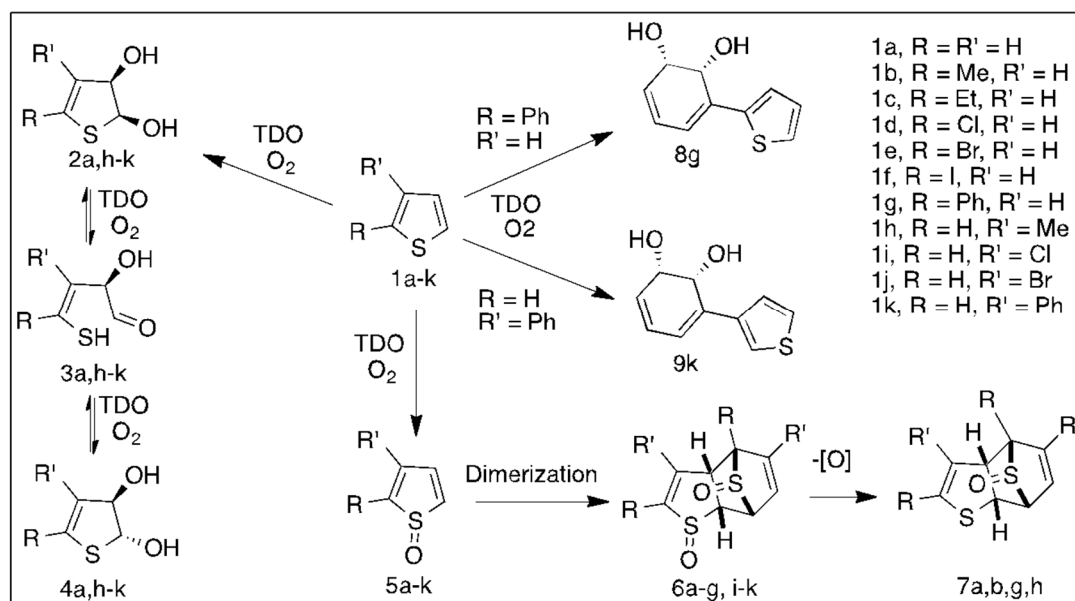
Scheme 2. TDO-catalyzed metabolism of thiophenes 1a-k.
