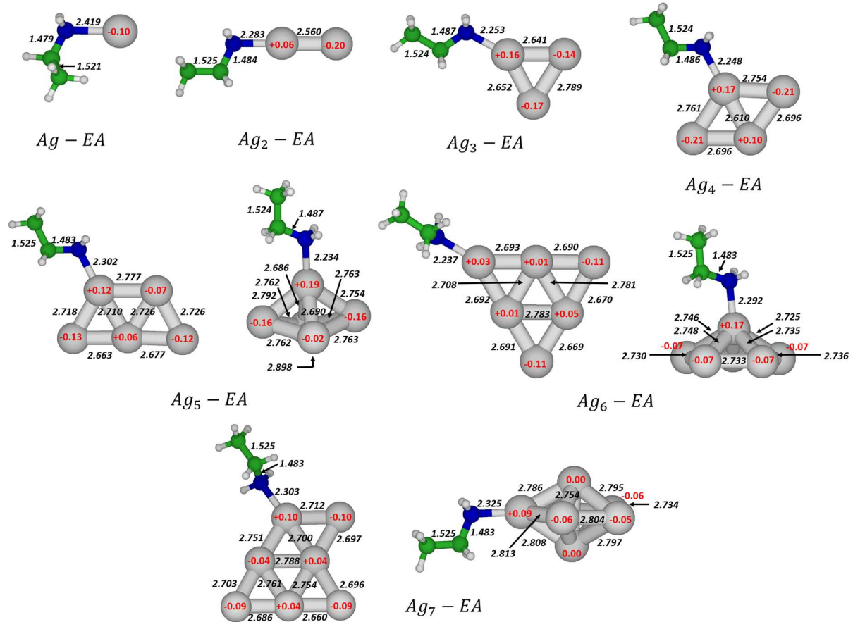
Figure 5. Most stable geometries of Ag_n^{2D} - EA and Ag_n^{3D} - EA calculated in the present work. Bond lengths (in Å, in black) and QTAIM atomic charges (in e , in red). OptB86b- \nu dW level of calculation.
