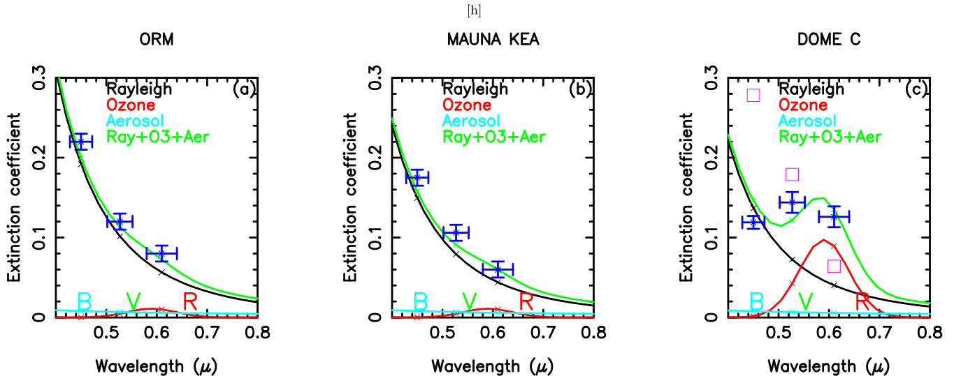
Figure 3. Atmospheric extinction (green line) at the three sites ORM (a), Mauna Kea (b), and Dome C (c), deduced from the respective contribution of the Rayleigh scattering (black line), ozone absorption (red line), and aerosol absorption (blue line). B , V , and R letters correspond to the respective wavelength centre in each filter band: 0.450, 0.527, and 0.610 \mu\text{m} . Blue + refers to measured atmospheric extinction.
