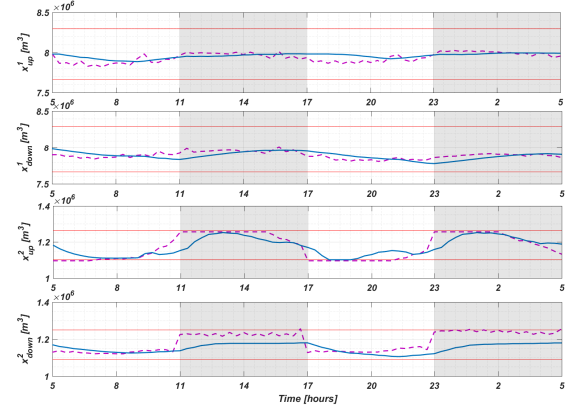
Figure 8: State estimates (purple dash-dot lines) and computed states (blue solid lines) for Scenario II
