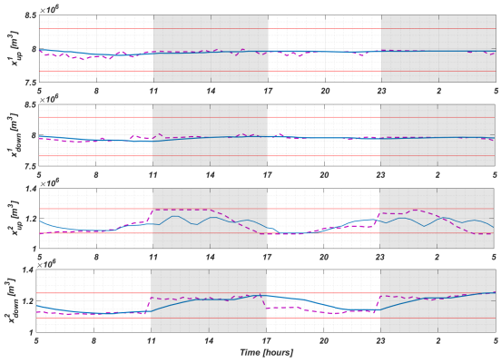
Figure 9: State estimates (purple dash-dot lines) and computed states (blue solid lines) for Scenario III
