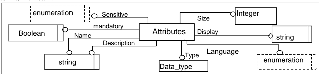
Figure 6: attribute properties
