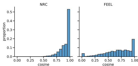
Figure 7: Distribution of cosine similarities with the NRC and FEEL lexicons.
