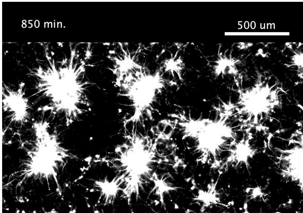
Movie S5: Time-lapse epifluorescence microscopy of microtubules displaying local contractions. Associated to Figure 2 in the main text. 1.5 % pluronic, [ATP] = 100 \mu\text{M} .
