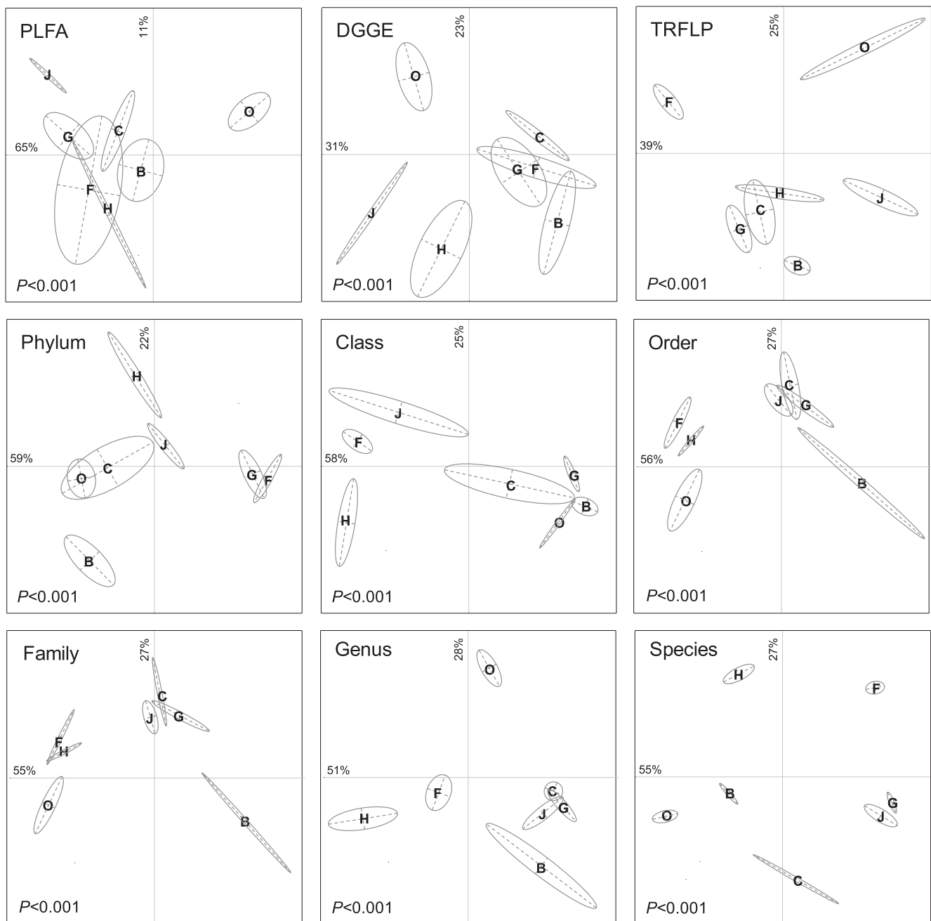
Fig. 2. Differences in bacterial community structure represented by Between Class Analysis (BCA) based on PLFA, TRFLP, DGGE or amplicon sequencing (Phylum to Species level) matrices. Grey lined ellipses represent the variability of each treatment (B: unfertilized; C: Ca(NO 3 ) 2 ; F: straw; G: straw + Ca(NO 3 ) 2 ; H: Green manure; J: Farmacyard manure; O: Sewage sludge). Letter represent the barycenter of the replicates (n = 3) for each treatment. Monte Carlo test revealed significant differences among treatments (simulated P < 0.001) for all methods. (For interpretation of the references to colour in this figure legend, the reader is referred to the web version of this article.)
