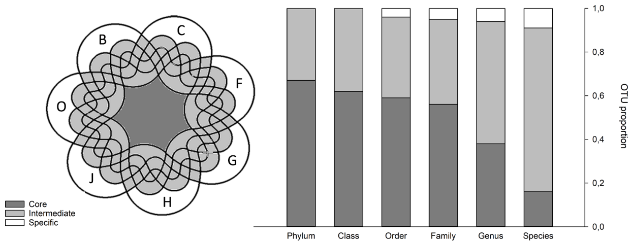
Fig. 4. Symmetric 7-way “Adelaide” Venn diagram (Grünbaum, 1992) depicting the core microbiota (dark grey), OTUs partially shared among 2 to 6 treatments (grey) and OTU specific to a treatment (B: unfertilized; C: Ca(NO 3 ) 2 ; F: straw; G: straw + Ca(NO 3 ) 2 ; H: Green manure; J: Farmyard manure; O: Sewage sludge). Stack bars representing the proportion of OTU distributed in the core, intermediate from the phylum to species level. Only OTUs found at least in 67% of the replicates (2/3) were considered. (For interpretation of the references to colour in this figure legend, the reader is referred to the web version of this article.)
