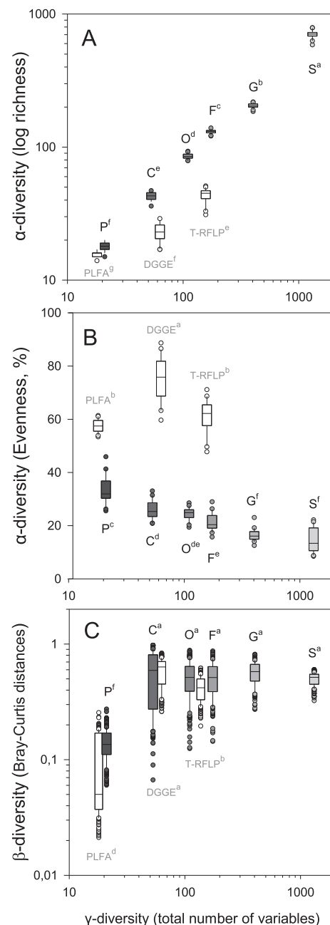
Fig. 1. Richness (A) and Evenness (B) of all samples ( n = 21 ) and Bray-Curtis inter-group distances (C; n = 128 ) as function of the number of variables obtained with molecular fingerprints (white boxes) or amplicon sequencing (grey boxes) at different taxonomy levels (P: Phylum; C: Class; O: Order; F: Family; G: Genus; S: Species). Different lowercase letters indicate significant ( P < 0.05 ) differences among methods.
