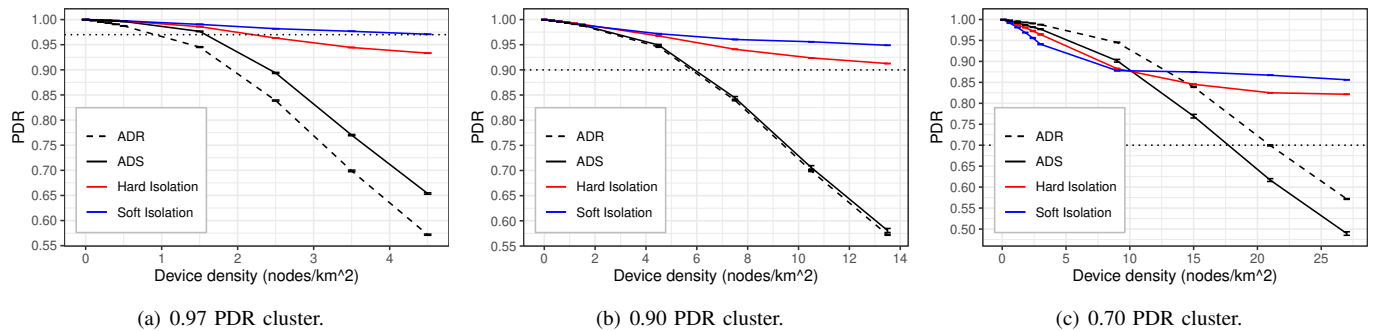
Fig. 2. PDR performance of devices in different clusters. The device densities for each plot is related to the number of devices of the associated cluster.
