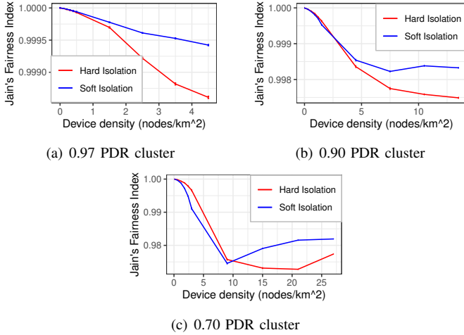
Fig. 5. Inter-device fairness of the PDR in each cluster computed with the Jain's Fairness Index (JFI). Maximum fairness is 1 and minimum is 1/n , with n being the number of participants.
