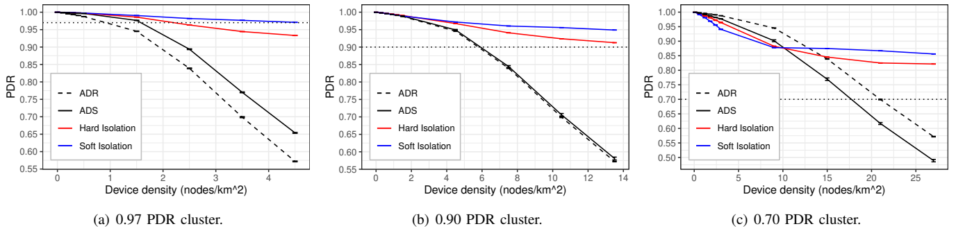
Fig. 2. PDR performance of devices in different clusters.
