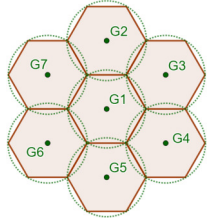
Fig. 1. Placement of gateways and devices in simulations.
