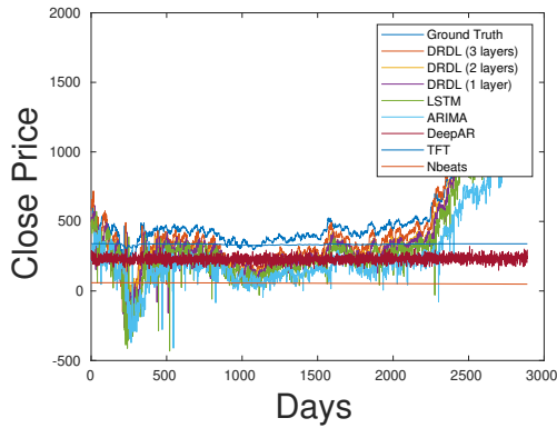
(b) RELIANCE
