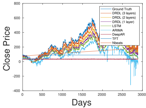
(c) TATAMOTORS
