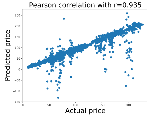
(a) AAPL
