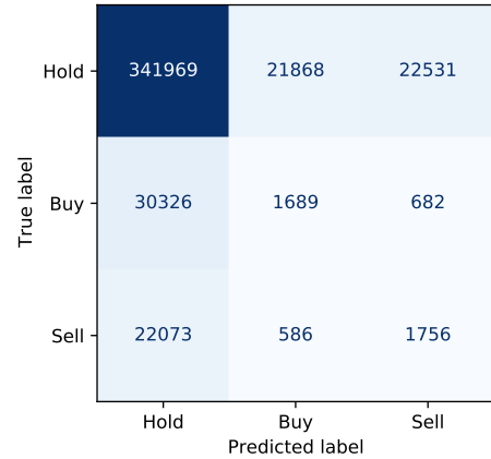
(f) LSTM
