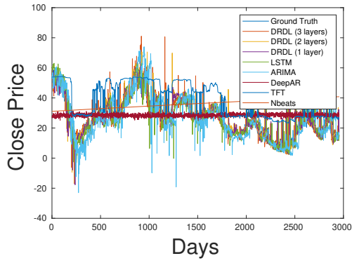
(a) ANF
