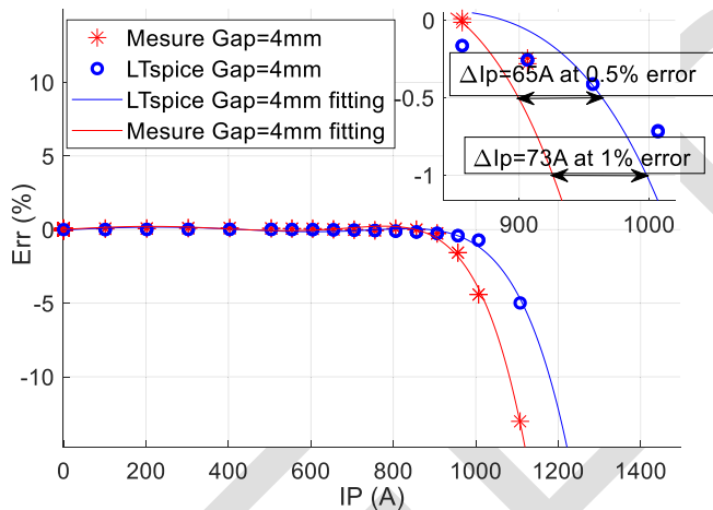
Fig. 14. Linearity for ASB core at I_{Pn} = 600 A. The magnetic circuit of an open loop Hall effect sensor is always designed according to the nominal current I_{Pn} and maximal current I_{Pmax} of a given application.
