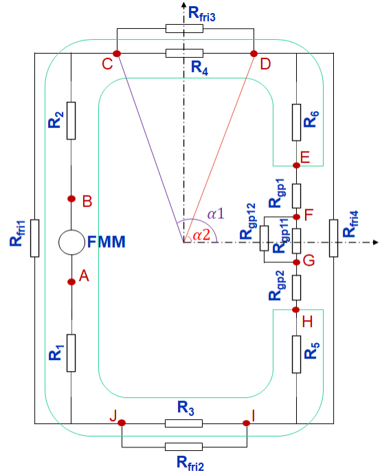
Fig. 5. Generic reluctance network topology applied to the ALB geometry. This topology will reproduce the flux density distribution inside the core and in the air-gap and the distribution of the fringing field in the air area around the magnetic core.
