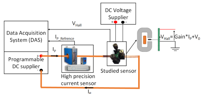
Fig. 12. Linearity test bench functioning principle. The DAS applies an increasing current profile through the DC suppliers. The applied current is measured by the high precision current sensor and by the tested sensor through its Hall die placed in the centre of the air-gap. The Hall die was calibrated accordingly to the magnetic circuit. The DAS collects the measurements for data post-processing.
