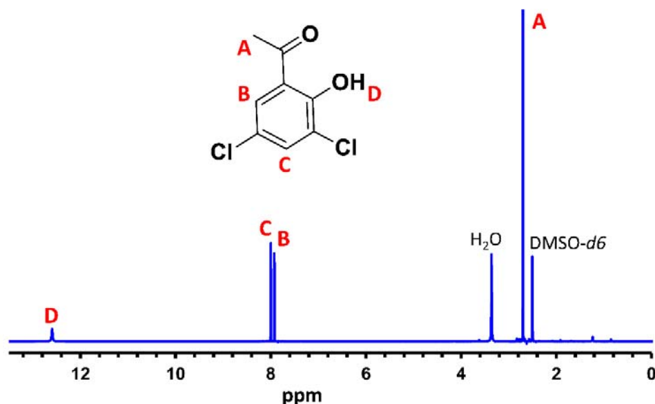
Figure S3. 1 H NMR spectrum of DCHA in DMSO- d 6 .
