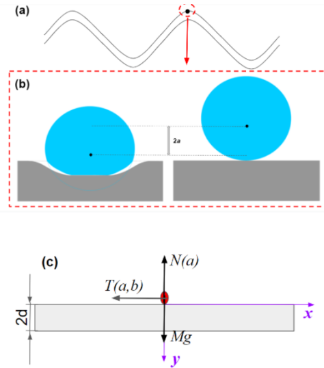
Figure 1: (a) Small ball pressed against a plate is excited by the Lamb wave (plate's deformation is highly exaggerated). (b) Zoom on the Hertz-Mindlin CAN. (c) Physical problem formulation for Hertz-Mindlin contact acoustic nonlinearity.
