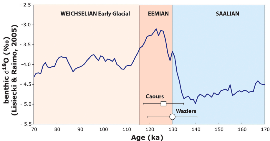
Fig. 5. Geochronological correlation of the obtained ESR/U-series mean ages for two Eemian sites of northern France (Caours and Waziers) with the Marine isotopic record of Lisiecki and Raimo (2005).
