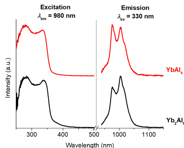
Figure 5. Corrected and normalized excitation and emission spectra of \text{YbAl}_4\text{Na} and \text{Yb}_2\text{Al}_8\text{Na}_2 in the solid state measured at room temperature.
