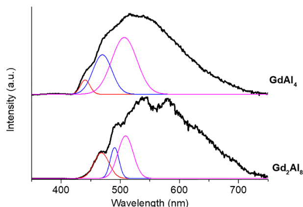
Figure 7. Corrected and normalized phosphorescence spectra of GdAl 4 Na and Gd 2 Al 8 Na 2 acquired in the solid state upon excitation at 330 nm and applying a 200 \mu\text{s} delay for the collection of the signal after the excitation flash at 77 K (black traces). 0–0 (red), 0–1 (blue) and 0–2 (magenta) phonon transitions were fitted with a Gaussian function.
