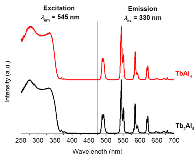
Figure 4. Corrected and normalized excitation and emission spectra of \text{TbAl}_4\text{Na} and \text{Tb}_2\text{Al}_8\text{Na}_2 measured in the solid state at room temperature.
