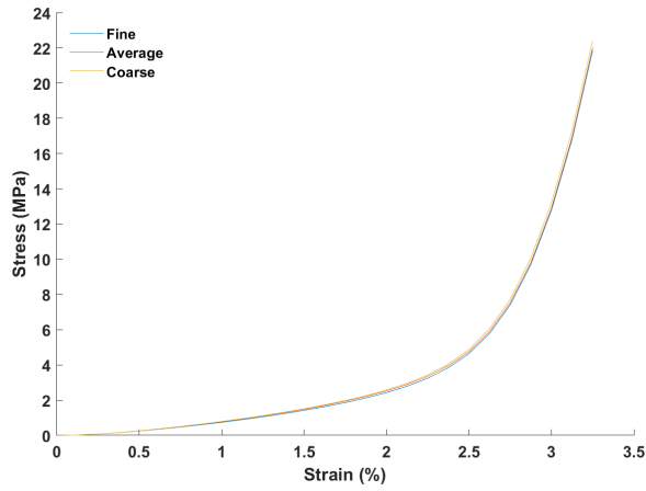
Figure 17. Mesh density sensitivity analysis on a SRVE of side length 1 mm with 6.6% of type A spherical inclusions: stress-strain relationship. (Type A monodisperse spheres.)
