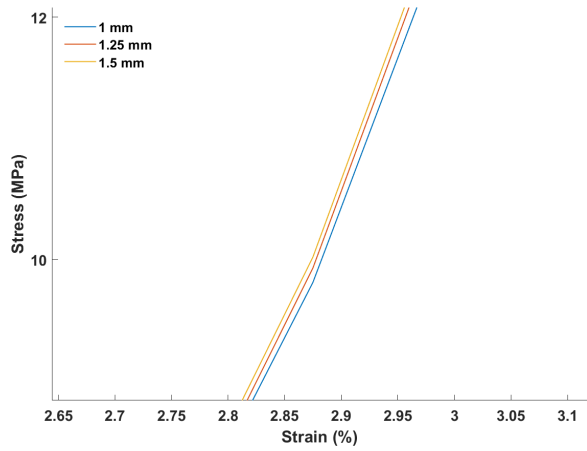
Figure 20. SRVE size sensitivity analysis for SRVEs with 6.6% of type A spherical inclusions with average mesh density: detail of stress-strain relationship.
