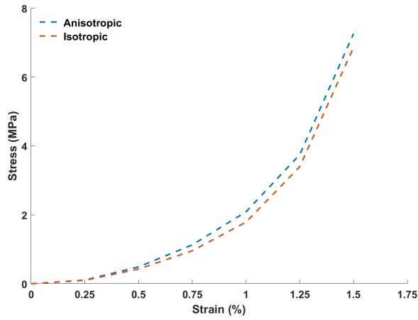
Figure 11. Comparison between the analytical result obtained with and without isotropization of Hill's tensor for PU with 2% porous inclusions.
