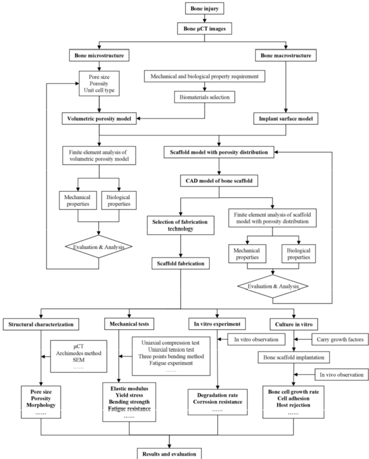
Fig. 3 BTE scaffolds: design, evaluation and fabrication. \mu CT (micro-computed tomography) [141].
