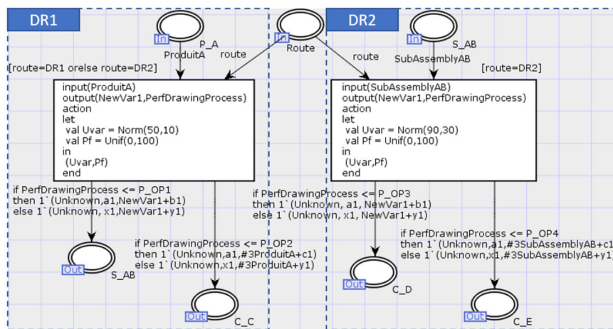
Figure 10 GCSPN for disassembly activity
