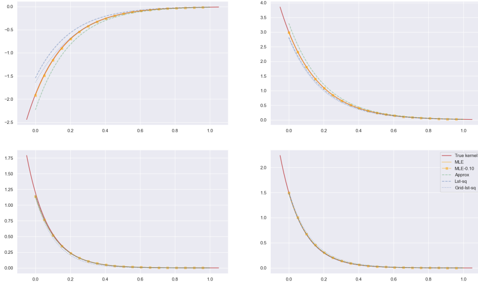
Figure 10: Reconstruction of interaction functions h_{ij} for Scenario (1) of two-dimensional Hawkes processes along with all estimated functions \hat{h}_{ij} . The real function is plotted in red and 25 estimations are averaged for each method.
