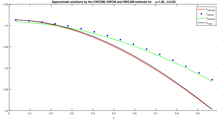
Figure 6: Approximate solutions of the CWCQM, HWCAM and HWCAM methods for \alpha = 1.85, \beta = 0.85
