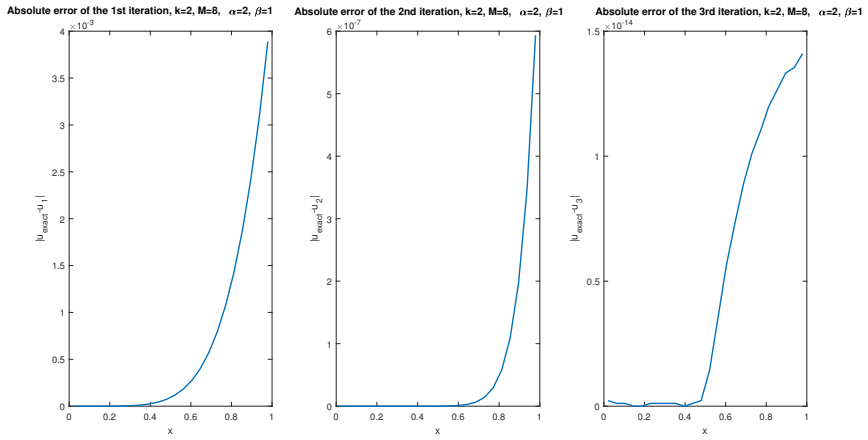
Figure 2: (2a) u_{CWQCM} for different values of \alpha, \beta with k = 2, M = 8 , (2b) Absolute errors of different iterations for \alpha = 2, \beta = 1, k = 2, M = 8 (b) in Eq (31) n = 5 .
