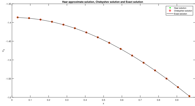
Figure 5: (5a) Absolute errors of Haar and Chebyshev approximate solutions (3rd iteration), J = 3 , for Haar, k = 2 , M = 8 for Chebyshev approximate solutions, Haar and Chebyshev approximate solutions (3rd iteration) and Exact solution, (5b) J = 3 , for Haar, k = 2 , M = 8 for Chebyshev solutions in Example 5.3
