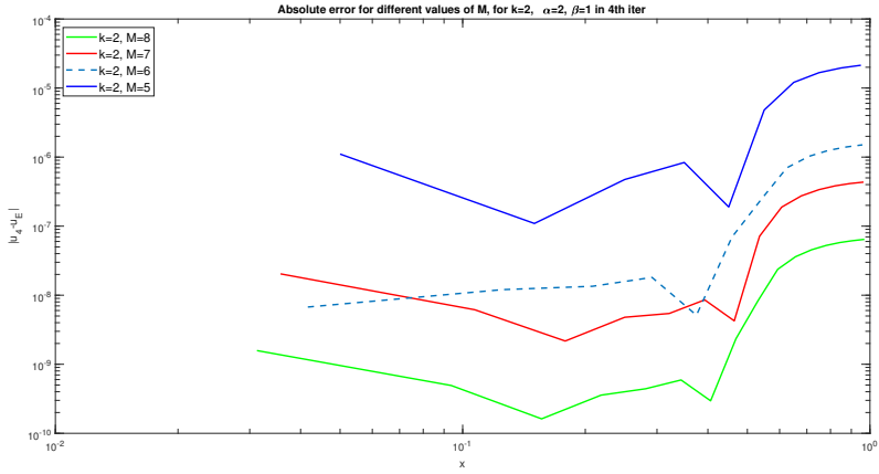
Figure 4: (4a) Absolute errors of different iterations for \alpha = 2, \beta = 1, k = 2, M = 8 , (4b) Absolute error for different values of M with k = 2, \alpha = 2, \beta = 1 in Example 5.2
