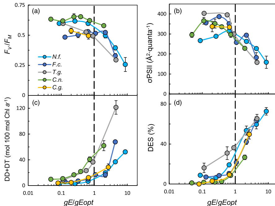
FIGURE 6 The dark-acclimated quantum yield of photosystem (PS II) ( F_V/F_M ) (a), the apparent size of PSII antenna functional cross-section ( \sigma_{\text{PSII}} ) (b), the sum of xanthophyll pigments diadinoxanthin (DD) and diatoxanthin (DT) (c) and the de-epoxidation state (DES) of the xanthophyll pool (d) plotted versus the dimensionless ratio between growth light ( gE ) intensity and gE for maximal growth rate ( gE/gE_{\text{opt}} ), where the vertical dashed line represents gE/gE_{\text{opt}} = 1 , in the five Arctic diatom species studies. All data points are triplicate mean \pm SD. Species abbreviations are found in Table 1. Fucoxanthin, chlorophyll c and \beta -carotene content are shown in Figure S10
