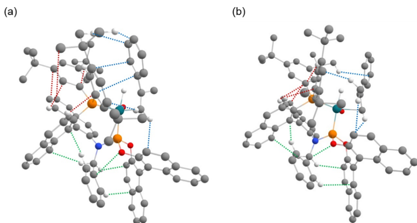
Fig. 2 Transition state geometries for the migratory insertion with coordination of the substrate through the si - (A) and re -faces (B). The figure shows the found NCIs. Ligand-ligand interactions are shown in red, substrate-ligand in blue and Bn group-ligand in green. Hydrogen atoms, wherever possible, are omitted to ensure better clarity.
