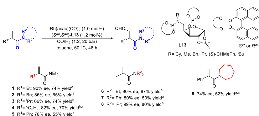
Scheme 9 Rh-catalyzed asymmetric hydroformylation of \alpha -substituted acrylamides with sugar-based phosphite-phosphoramidite ligands L7 . a Ligand ( S^{ax} , S^{ax} )- L13 ( R = \text{Cy} ) was used. b Ligand ( S^{ax} , S^{ax} )- L13 ( R = (S)\text{-CHMePh} ) was used. c Temperature = 90 °C for 16 h.
