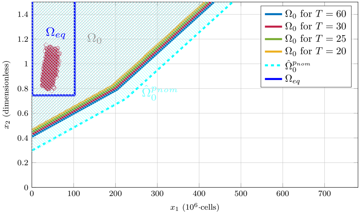
Figure 2: Probabilistically certified sets \Omega_0 for different horizons T (days). The red circles are the benign equilibrium points of model (1) for 1000 parameters vector samples.
