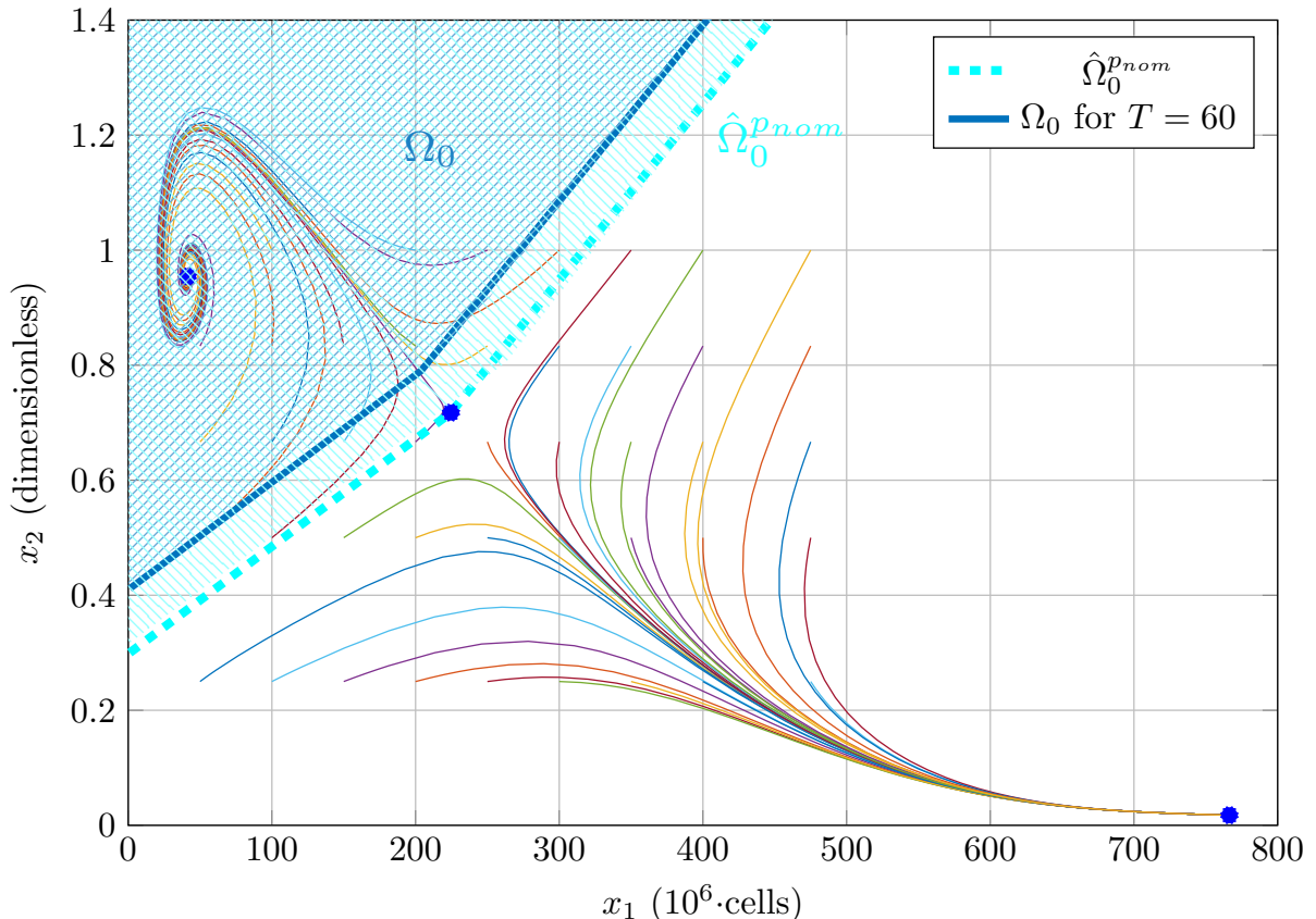
Figure 3: Phase portrait of (1), the colored trajectories represent the states (x_1, x_2) for different initial conditions, the blue dots correspond to the 3 equilibrium points of the system, estimated nominal uncontrolled RoA \hat{\Omega}_0^{p_{nom}} in dashed cyan and the estimated certified initial target set \Omega_0 for T = 60 in blue.
