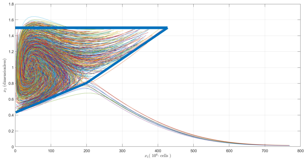
Figure 4: Monte-Carlo simulations to validate the certified target set \Omega_0 .
