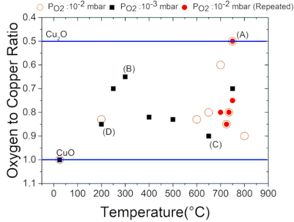
Figure 1. Oxygen to copper ratio in \text{Cu}_x\text{O} v.s temperature at 10^{-2} mbar and 10^{-3} mbar oxygen partial pressures (estimated from RBS measurements).
