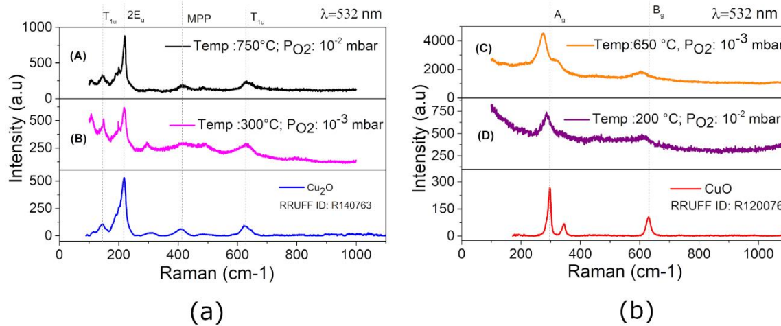
Figure 2. Raman spectra of (a) A and B (b) C and D deposited at different temperatures and oxygen partial pressures on quartz along with the references from RRUFF database translated for viewing purpose (excitation wavelength = 532 nm).
