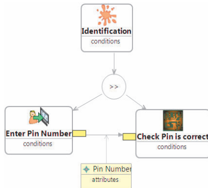
Figure 2. Tasks relationships in HAMSTERS
