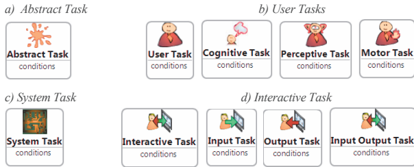
Figure 1. Illustration of the task type within HAMSTERS
