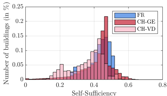
Figure 3: Histogram of the self-sufficiency rate of the buildings in the three administrative region of the GGA. Blue - French region (FR) ; dark red - canton of Geneva (CH-GE); light pink - canton of Vaud (CH-VD)
