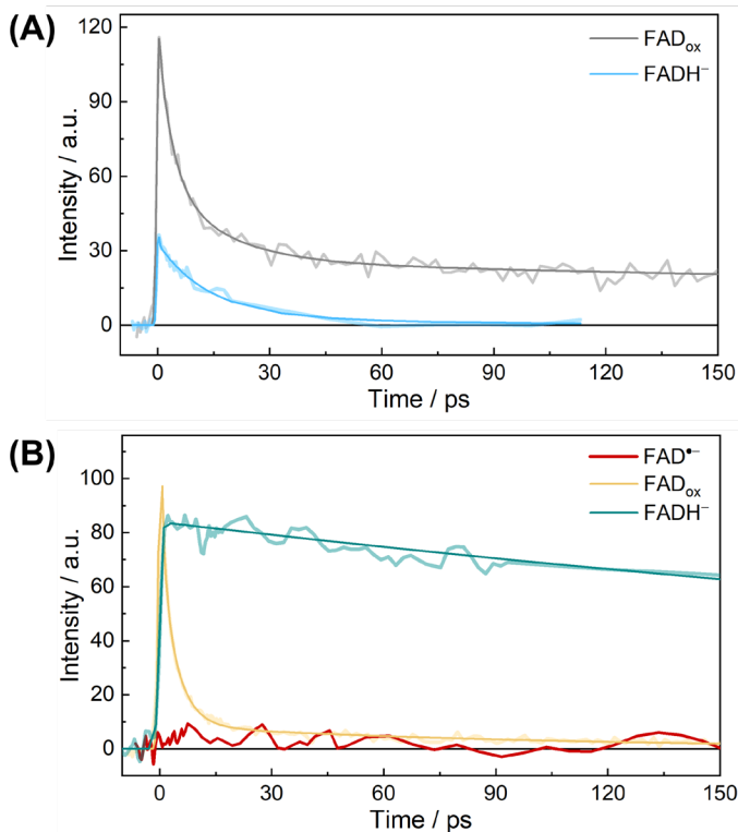
Fig. 4 Fluorescence decay on the picosecond timescale of free \text{FAD}_{\text{ox}} and \text{FADH}^- in solution (A) and of \text{FAD}^* , \text{FAD}_{\text{ox}} and \text{FADH}^- in GOX. For \text{FAD}_{\text{ox}} the decay on the timescale of a few picosecond is assigned ET to the isoalloxazine ring system, in solution from adenine to which it is stacked in a fraction of the flavins, in GOX from closely tyrosine. For \text{FADH}^- in solution the decay is assigned to a conical intersection with the ground state reached by conformational flexibility of the isoalloxazine ring system. This conical intersection is thought to be more difficult to reach in a constrained protein environment, as in GOX. Panel B is reprinted with permission from Ref. 4 . Copyright 2022 the Authors.
