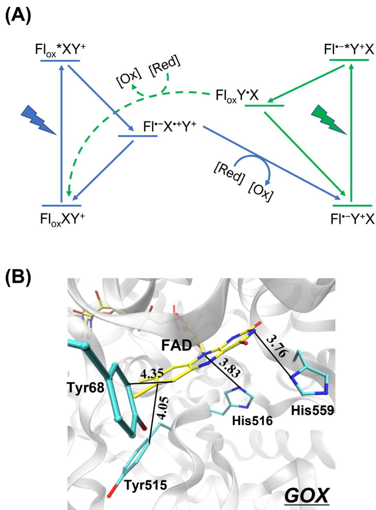
Fig. 6 A. General reaction pathways for photoinduced ET in flavoproteins that include the proposed cycle of the photooxidation of Fl^- . X stands for the electron-donating residue (tryptophan or tyrosine) and Y^+ represents the electron-accepting residue (presumably histidine or arginine) in the protein active site. [Red] and [Ox] represent external reductants and oxidants. An exchange mechanism between reduced free flavins and protein-bound Fl_{ox} has also been proposed to explain the accumulation of protein-bound Fl^- under light illumination in the presence of hole scavenger 65 , which is not included in the present scheme. B. Active site in the crystal structure of GOX from Aspergillus niger (PDB entry: 1CF3). The presence of electron-donating tyrosines and tryptophans, as well as electron-
