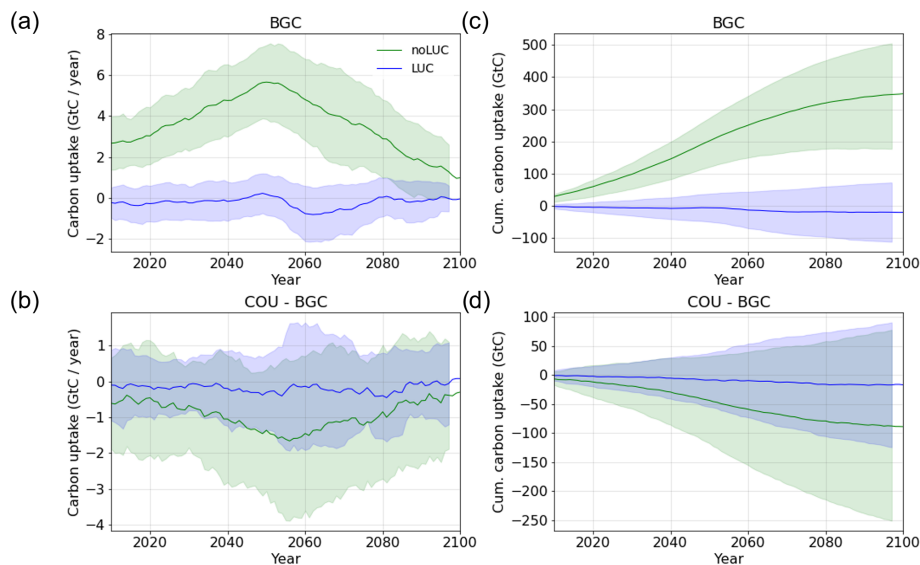
Figure 4. Interannual variation of global (a, b) land carbon uptake and (c, d) cumulative carbon uptake in LUC-concentrated and noLUC ecosystems given as mean and standard deviation (shaded area) of five ESMS and three approaches. Panels (a) and (c) show BGC simulation outputs, and panels (b) and (d) show the difference in COU and BGC simulation outputs.
