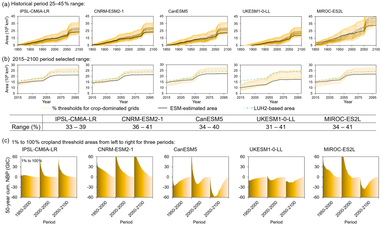
Figure A2. (a) The cropland-fraction thresholds ranging from 25 % to 45 % of the grid box area analyzed in the sensitivity study and (b) the selected (resultant) range of thresholds for identifying the energy-crop-concentrated area with the selected range for each ESM indicated in the table. Panel (c) shows the cumulative NBP of the areas corresponding to the range of cropland thresholds from 1 % to 100 % (left dark to right light color) in three periods.
