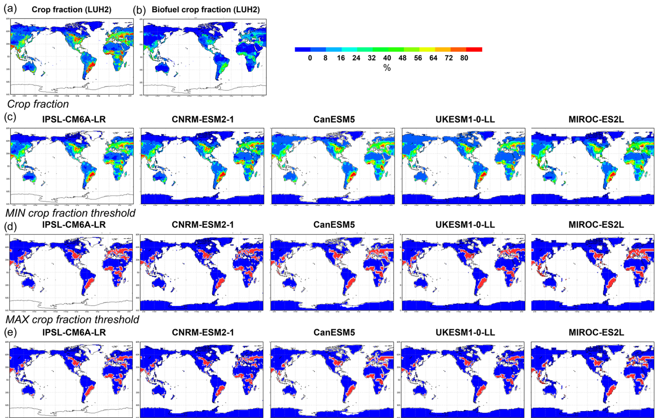
Figure A3. Spatial variation of (a) grid cropland fraction (b) and second-generation bioenergy cropland fraction by LUH2. Panel (c) shows the spatial variation of grid cropland fraction estimated by CMIP6 ESMs. The spatial variation of the selected (d) minimum and (e) maximum thresholds (which intersect at least once either the global cropland area estimated by ESM itself or LUH2 data set from 2015 to 2100 as shown in Fig. A1) for estimating crop-concentrated grids in 2100.
