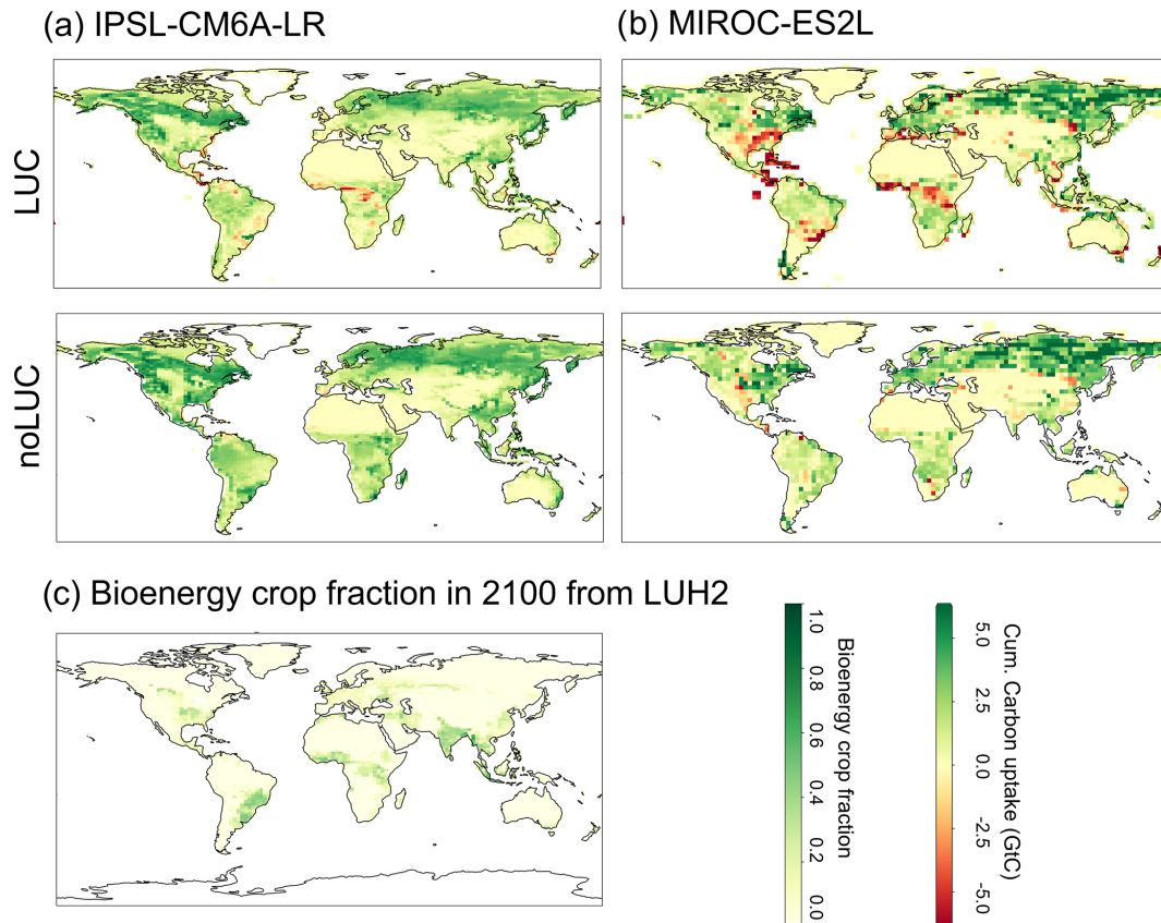
Figure 5. Spatial variations of the cumulative over 2040–2100 period carbon uptake by (a) IPSL-CM6A-LR and (b) MIROC-ES2L given for the fully coupled simulations with and without LUC. The negative values indicate less sink/larger source from land to atmosphere. (c) The bioenergy crop area in 2100 from LUH2.
