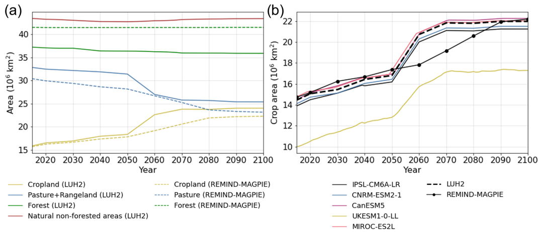
Figure 1. Time series of (a) the changes in the area of croplands, pastures, and forests according to REMIND-MAGPIE and LUH2, and (b) the area of croplands in LUH2, REMIND-MAGPIE, and five CMIP6 ESMs under the SSP5-3.4-OS pathway. In panel (a), pastures and rangelands of LUH2 are treated together as pastures.
