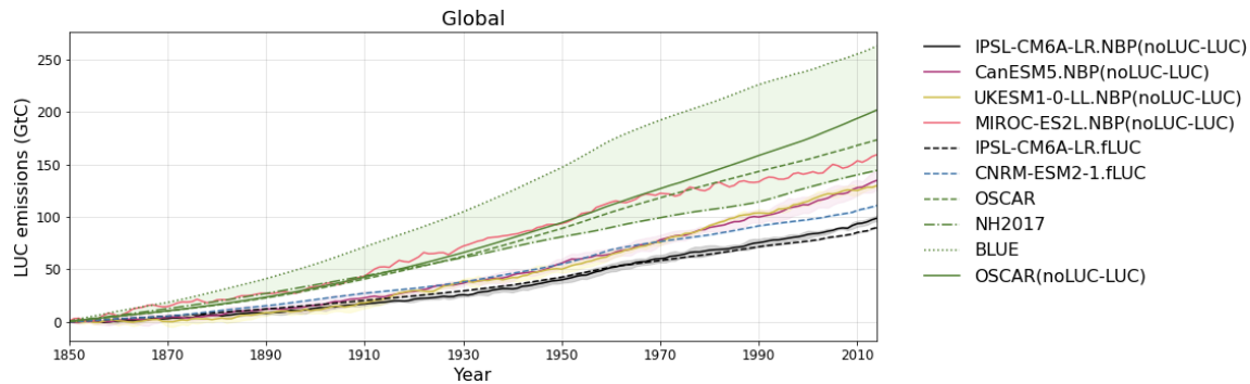
Figure 2. Evaluation of cumulative global LUC emissions by ESMs against three bookkeeping models. LUC emissions are defined by two methods: (1) the difference in NBP between simulations with and without LUC (solid lines) and (2) the “fLUC” variable provided in CMIP6 (dashed lines). The estimates of the bookkeeping approach using OSCAR are shown for cases with (noLUC-LUC) and without LASC. The range of bookkeeping models is shaded green.
