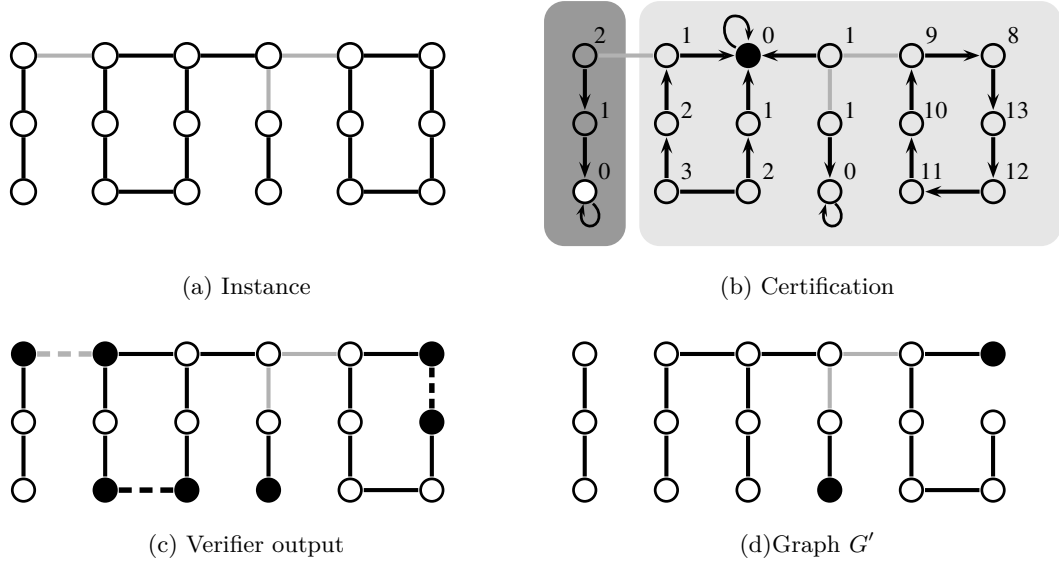
Figure 2 Construction in the proof of Theorem 19. (a) Illustration of an instance. The black edges are the edges described in \ell (in this example, \ell is a proper encoding of a set of edges), and the gray edges are the other edges of the graph. Note that (G, \ell) is not in the languages as the set of black edges is neither connected, nor acyclic. (b) Illustration of a certificate assignment. The depicted numbers are the hop-distances, and the arrows provide the orientation of the pointers. The nodes in the light grey area have the ID of the black node as their root-ID in their certificates. The ones in the dark grey rectangle have the ID of the white node as their root-ID in their certificates. (c) Illustration of the rejecting nodes and edges. The black nodes are the ones that reject, and the dashed edges have both endpoints rejecting. The two top left black nodes reject because they do not have the same root-ID. The ones linked by a dashed edge at the bottom reject because they detect that the edge connecting them is in the input but is not oriented (that is, the condition “ p(w) = u ” does not hold). The third black node on the bottom rejects because it has a distance-counter equal to zero, and a pointer to itself, as if it was the root, but its ID is not the root-ID in its certificate. Finally, the endpoints of the dashed edge on the right reject because their distance counter are not consistent with the pointers. (d) The labeled graph (G', \ell') obtained after removing the edges whose both endpoints reject. The black nodes are the ones that reject when we run again the verifier on this labeled graph, with the same certificate.
