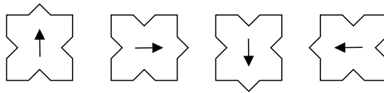
Figure 1: Flow tiles for \mathbb{F}_2 .
