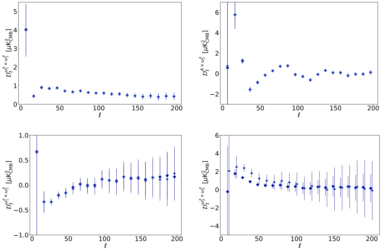
Fig. A.2. Best-fit values of the \mathcal{D}_\ell^{\omega_1^\beta \times \omega_1^\beta} (top left), \mathcal{D}_\ell^{A \times \omega_1^\beta} (top right), \mathcal{D}_\ell^{\omega_1^\beta \times \omega_2^\beta} (bottom left) and \mathcal{D}_\ell^{\omega_2^\beta \times \omega_2^\beta} (bottom right) moment parameters for the \beta -2 fitting scheme applied on the d1c simulation type (diamonds) and r\beta -2 on d1c (plus sign).
