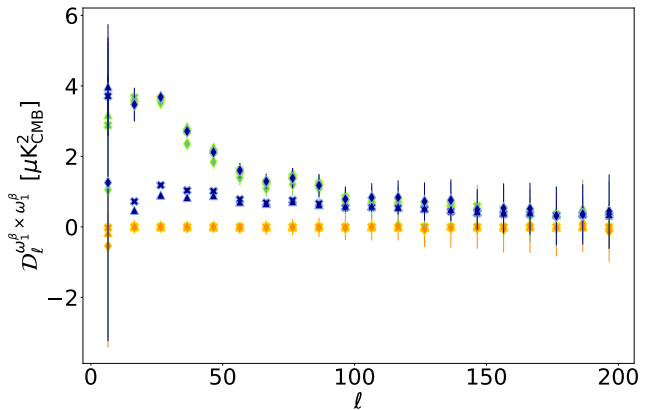
Fig. 6. Best-fit values of the first-order moment D_\ell^{\omega_1^\beta \times \omega_1^\beta} for d0 (orange), d1T (green), and d1 (blue), fitting with \beta -1 (crosses), \beta -2 (triangles), and \beta -T (diamonds).
