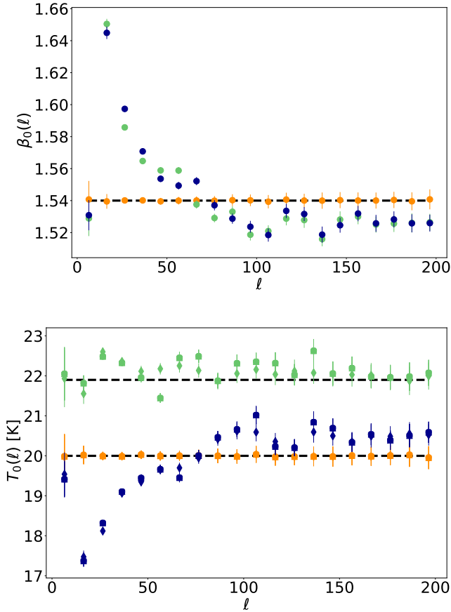
Fig. 4. Top: median of the best fit values of \beta_0(\ell) in d0 (orange), d1T (green), and d1 (blue) for the MBB (circles). \beta_{d0} is marked by the dashed black line. Bottom: same as above but with T_0(\ell) , the black dashed-lines being T_{d0} = 20 K and T_{d1T} = 21.9 K.
