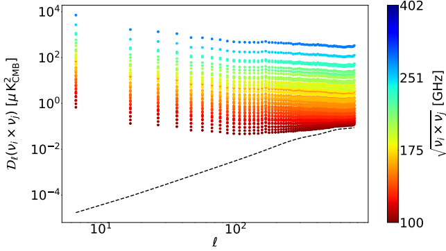
Fig. 1. Mean value over the N_{\text{sim}} simulations of the B -mode angular power spectra \mathcal{D}_\ell(v_i \times v_j) for the d1c simulation type, with r_{\text{sim}} = 0 . The color bar spans all the N_{\text{cross}} spectra \mathcal{D}_\ell(v_i \times v_j) , associated to their reduced cross-frequency \nu_{\text{red}} = \sqrt{v_i v_j} , from 100 GHz (dark red) to 402 GHz (dark blue). The input CMB lensing power spectrum is shown as a black dashed line.
