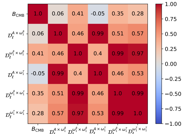
Fig. 12. Correlation matrices of the 2D-SED shapes of the CMB ( B_{\text{CMB}}(v_i \times v_j) ) and dust moments \mathcal{D}_\ell^{N \times M}(v_i \times v_j) in the (v_i, v_j) space. Each element represents the Pearson correlation coefficient between any 2 of these 2D-SED shapes. The correlation matrices are displayed in the case of the \beta-2 fitting scheme (top panel) and the \beta-T one (bottom panel).
