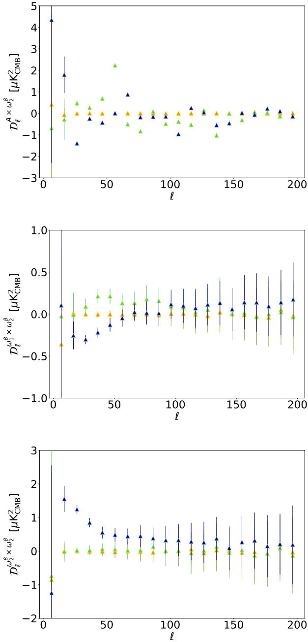
Fig. 7. Best-fit values of the second-order \mathcal{D}_\ell^{A \times \omega_2^\beta} , \mathcal{D}_\ell^{\omega_1^\beta \times \omega_2^\beta} and \mathcal{D}_\ell^{\omega_2^\beta \times \omega_2^\beta} moment parameters in d0 (orange), d1T (green), and d1 (blue) for \beta -2 (triangles).
