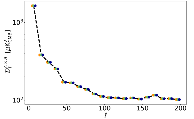
Fig. 5. Median of the best-fit values of D_\ell^{A \times A} for d0 (orange), d1T (green), and d1 (blue) using the MBB fitting scheme. The values for the three simulation types are shifted with respect to one another by \ell = 2 in order to distinguish them. The black dashed line is the amplitude power spectrum of the dust template map used to build the three simulation sets d0, d1T, and d1.
