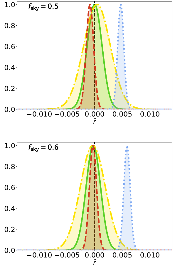
Fig. 10. Top panel: posterior on \hat{r} in the d1c simulation type on f_{\text{sky}} = 0.5 for the different fitting schemes: r\text{MBB} (blue, dotted line), r\beta -1 (red, dashed line), r\beta - T (green, solid line), and r\beta -2 (yellow, dash-dotted line). The vertical black dashed line marks the value of r_{\text{sim}} = 0 . Bottom panel: same, in the case of the d1c simulation type on f_{\text{sky}} = 0.6 .
