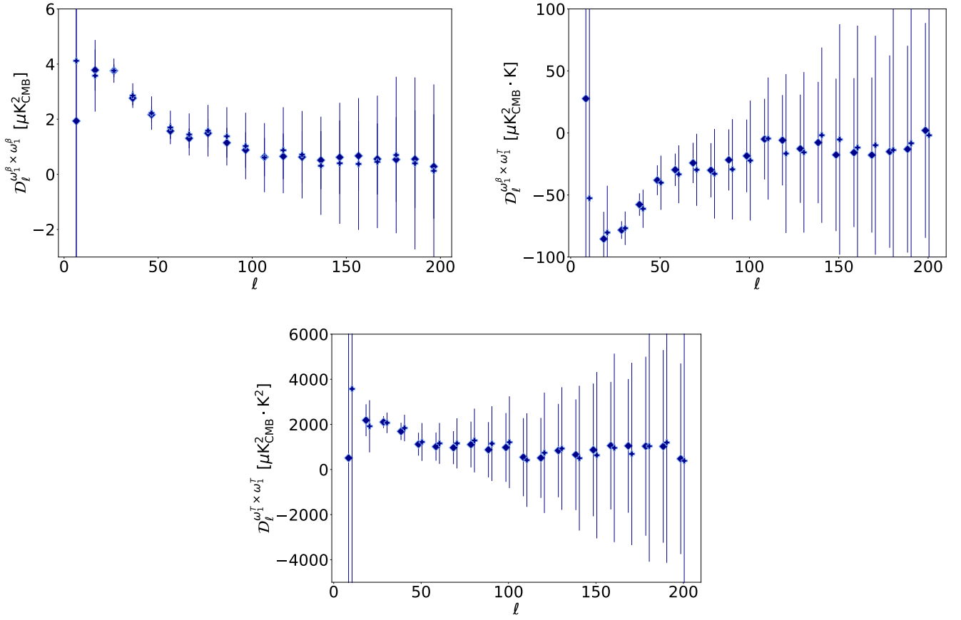
Fig. A.3. Best-fit values of the \mathcal{D}_\ell^{\omega_\beta^\beta \times \omega_\beta^\beta} (top left), \mathcal{D}_\ell^{\omega_\beta^\beta \times \omega_I^I} (top right) and \mathcal{D}_\ell^{\omega_I^I \times \omega_I^I} (bottom) moment parameters for the \beta - T fitting scheme applied on the d1c simulation type (diamonds) and r\beta - T on d1c (plus sign).
