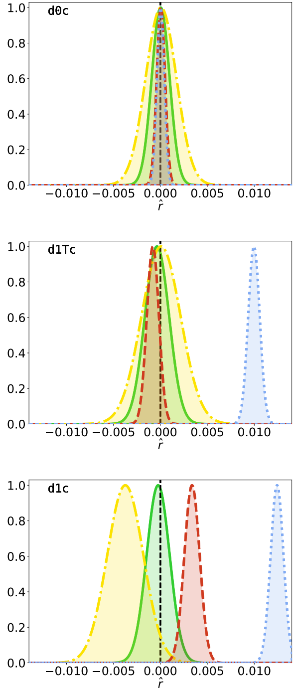
Fig. 9. Top panel: posterior on \hat{r} in the d0c simulation type for the different fitting schemes: r\text{MBB} (blue, dotted line), r\beta-1 (red, dashed line), r\beta-T (green, solid line), and r\beta-2 (yellow, dash-dotted line). The vertical black dashed line marks the value of r_{\text{sim}} = 0 . Central panel: same, but in the case of the d1Tc simulation type. Bottom panel: same, but in the case of the d1c simulation type.
