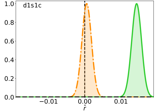
Fig. 13. Posterior on \hat{r} in the d1s1c simulation type with r_{\text{sim}} = 0 and f_{\text{sky}} = 0.7 for the different fitting schemes: r\beta - T (green, solid line) and sr\beta - T (orange, dash-dotted line). The vertical black dashed line marks the value r_{\text{sim}} = 0 .
