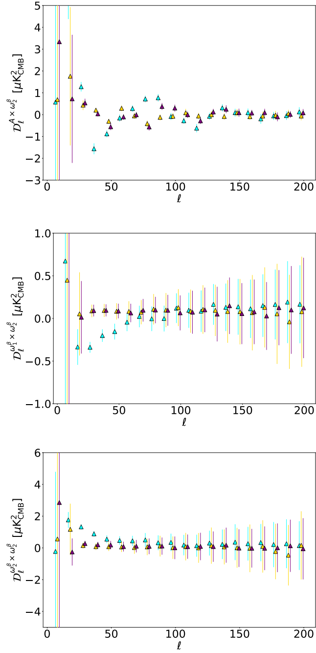
Fig. A.5. \beta - 2 moment coefficients for different f_{\text{sky}} : f_{\text{sky}} = 0.7 (cyan), f_{\text{sky}} = 0.6 (purple) and f_{\text{sky}} = 0.5 (gold).
